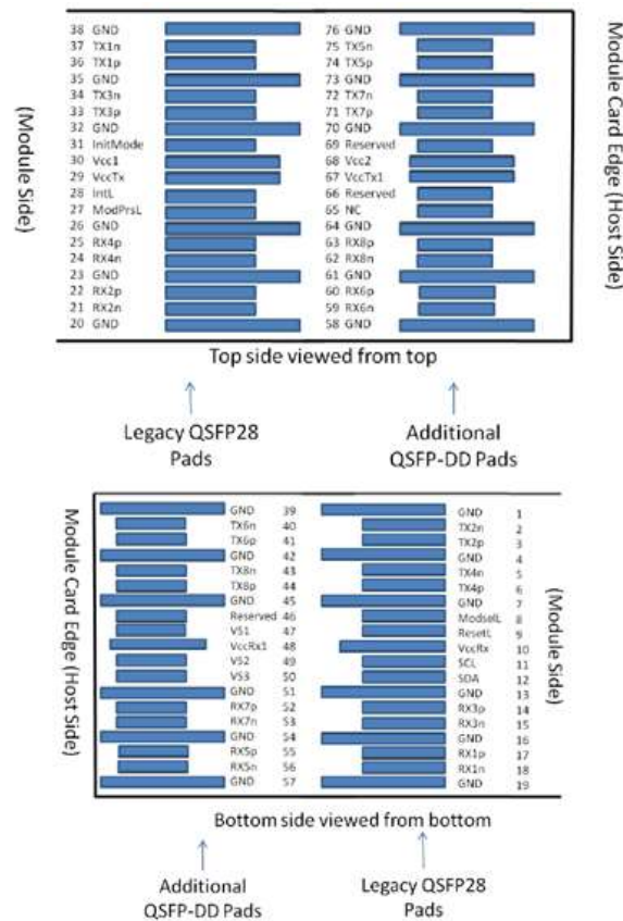
Figure 2. Electrical Pin-out Details
