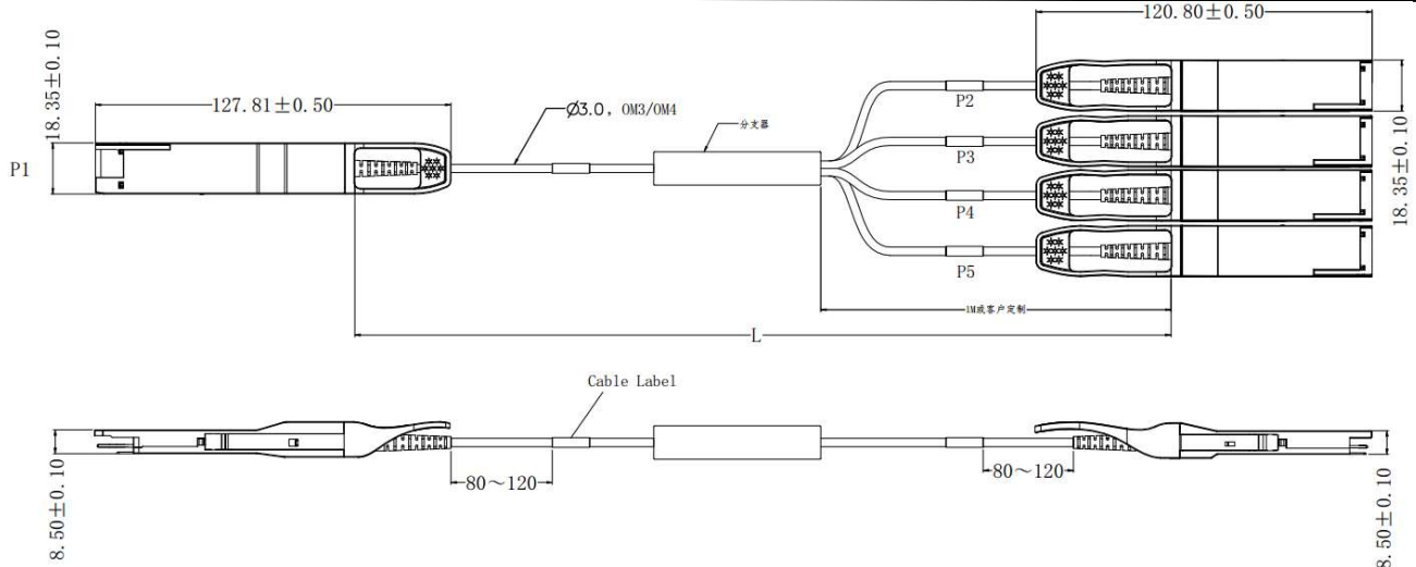
Figure 12. Mechanical Specifications
