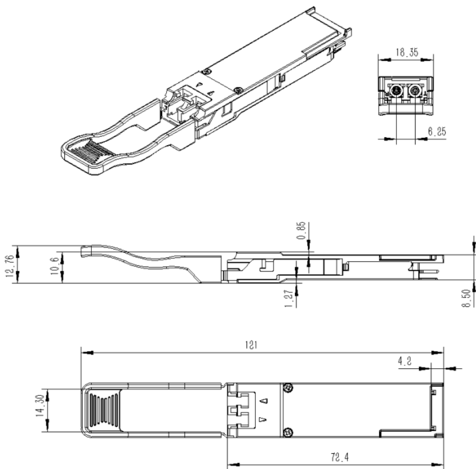
Figure 3. Mechanical Dimensions
